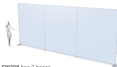
FW208 has 2 bases, 2 droop preventors, 2 - full uprights & 2 center supports, 2 - crossbars.
