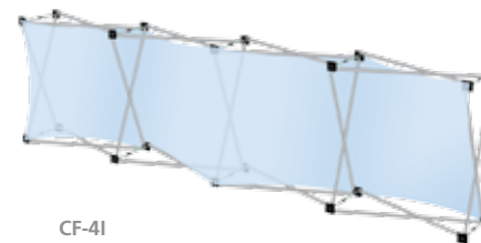
CF-4I 1 x 4 Front, Back, Front, Back, Single Slant 132.75" x 30.75"
