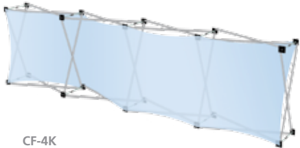
CF-4K 1 x 4 Front, Back, Front, Front, Single Slant 129.75" x 30.75"
